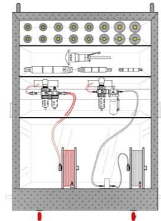
VISTA FRONTAL
